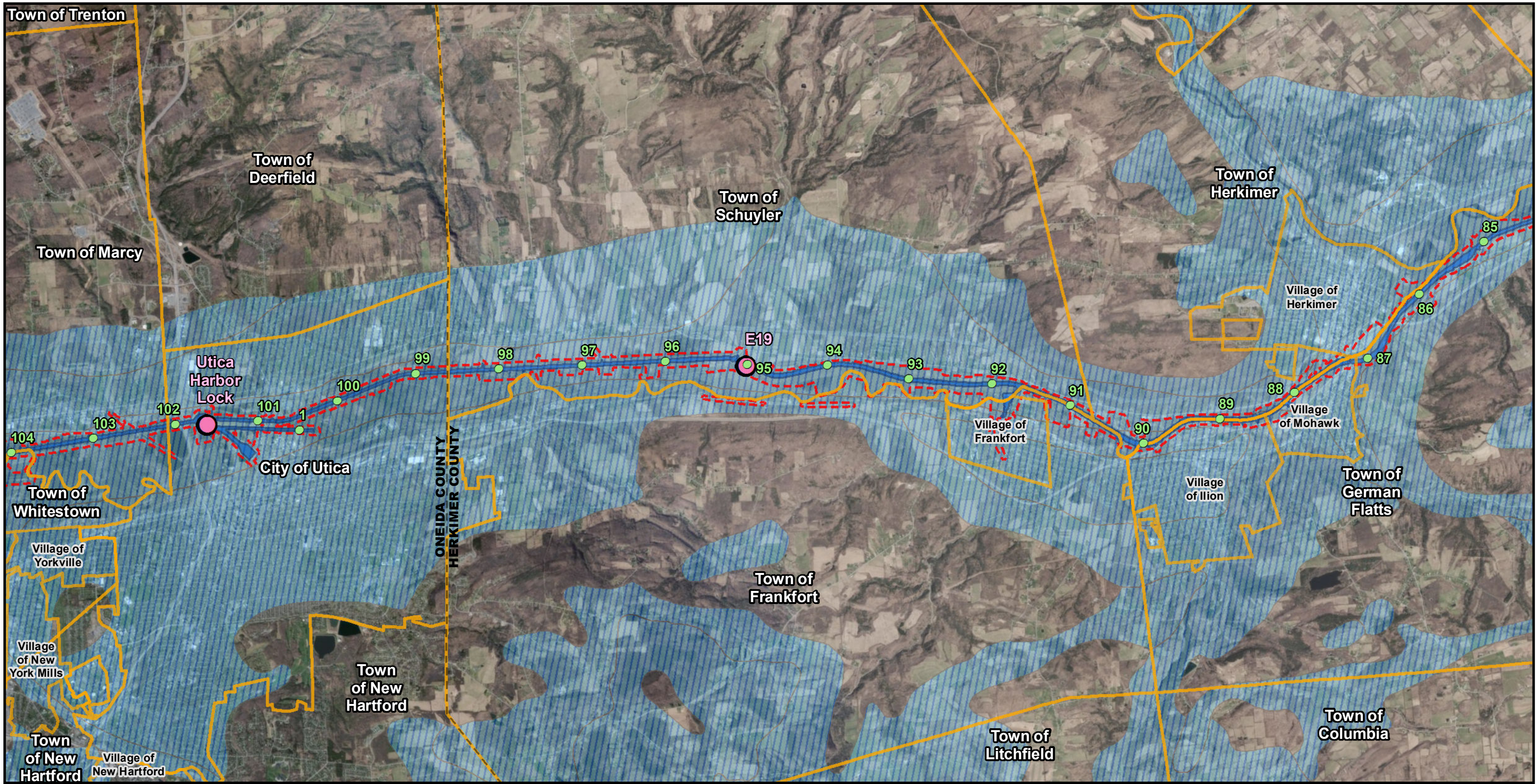
Figure 44F: Aquifers
